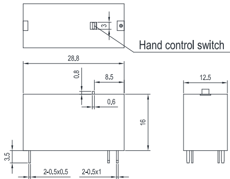
1A3/1B3 Outline Dimensions (Double coils latching)
