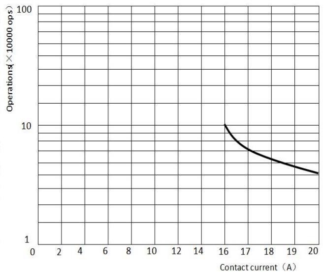
ENDURANCE CURVE
