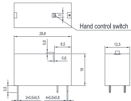
1A2/1B2 Outline Dimensions (Double coils latching)
