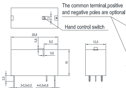
1A2/1B2 Outline Dimensions (Double coils latching)
