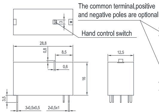
1A5/1B5 Outline Dimensions (Single coil latching)
