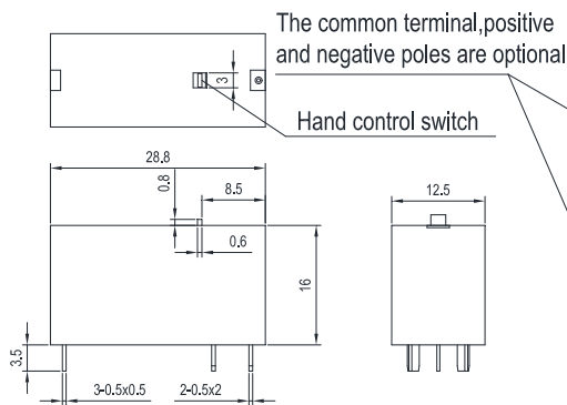
1A2/1B2 Outline Dimensions (Single coil latching)
