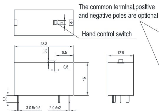
1C2 Outline Dimensions (Single coil latching)
