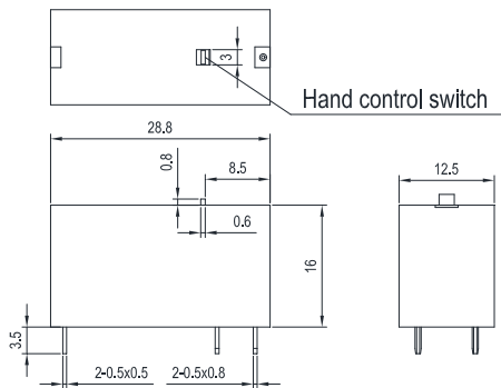
1A5/1B5 Outline Dimensions (Double coils latching)
