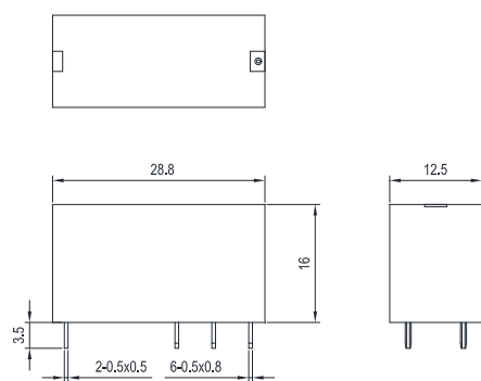
1C2 Outline Dimensions (Double coils latching)
