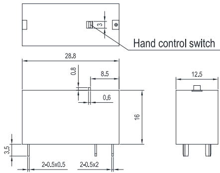
1A1/1B1 Outline Dimensions (Double coils latching)
