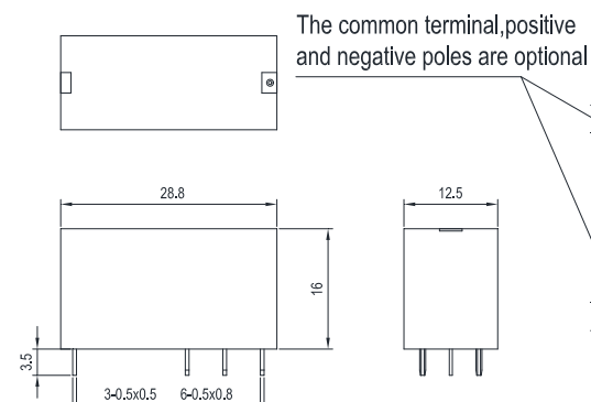
1C2 Outline Dimensions (Double coils latching)
