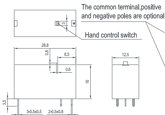
1A5/1B5 Outline Dimensions (Double coils latching)
