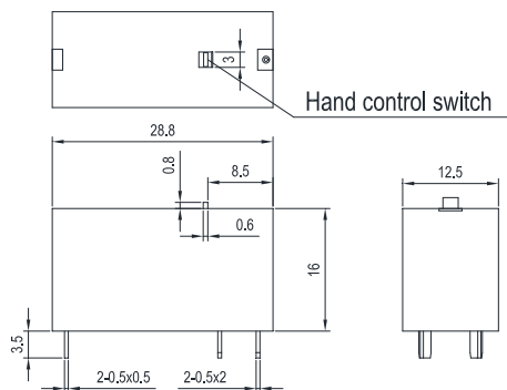
1A6/1B6 Outline Dimensions (Double coils latching)
