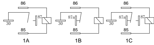
Wiring diagram (Bottom views)
