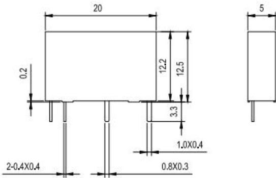
1A2 Outline Dimensions
