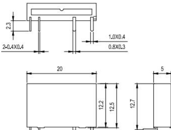
1A1 Outline Dimensions
