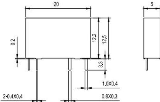
1A2 Outline Dimensions
